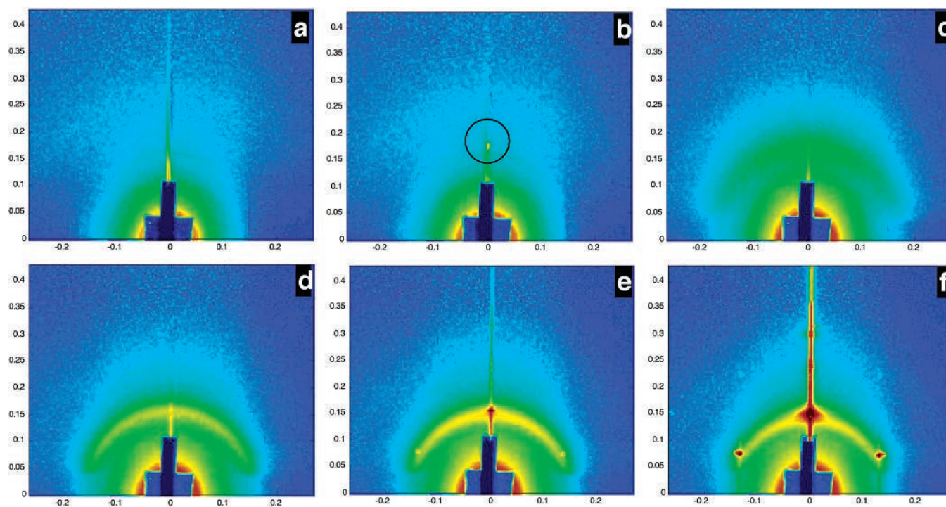
Figure 4. GISAXS patterns obtained after the specified times, t (seconds), are presented for sample 0.12, corresponding to the following: (a) the isotropic phase, (b) the lamellar mesophase, (c and d) the correlated micellar, and (e and f) the hexagonal mesophase.
