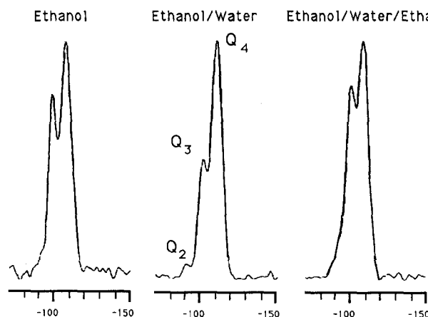
Fig. 7. ^{29}\text{Si} MAS NMR spectra for xerogels aged in ethanol, ethanol-water, and ethanol-water-ethanol.
